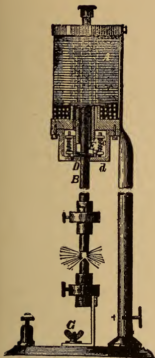
Fig. 22. THE BRUSH LIGHT.
